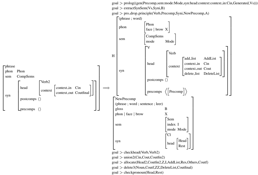
Figure 7: Last Complement Pronoun Rule
